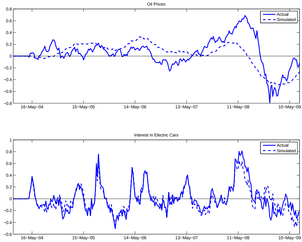
Figure 7 Simulation Using Only Shocks to Interest in Electric Cars, Subtracting the Values Predicted Without Shocks
